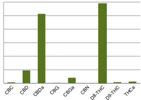
Cannabinoids (% weight)
